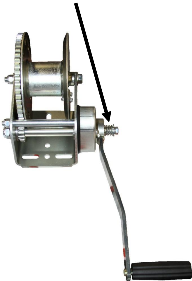
Single handle model spring, washer and bolt
